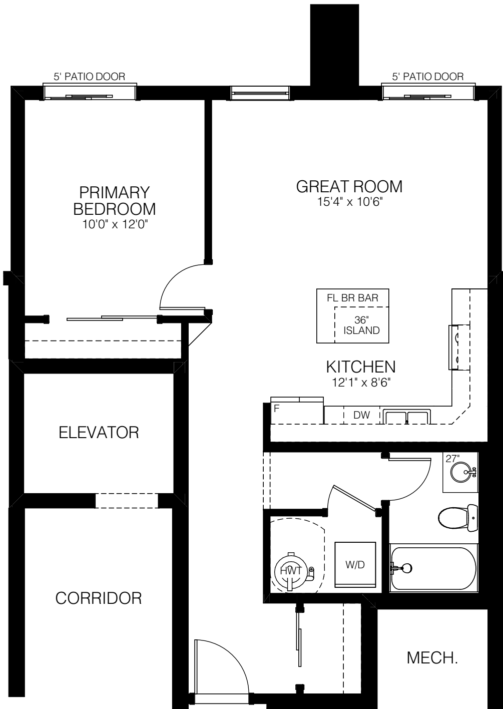
VANIER UNIT TYPE 'H' 707 SQFT
