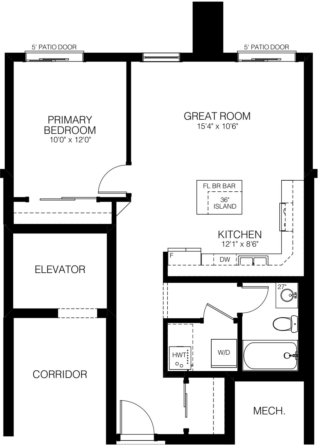
VANIER UNIT TYPE 'H' 707 SQFT
