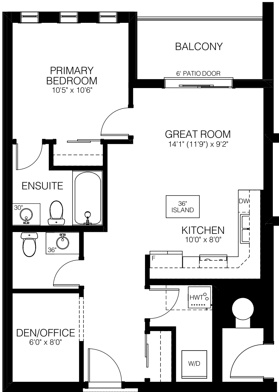
SERENITY UNIT TYPE 'G' 680 SQFT
