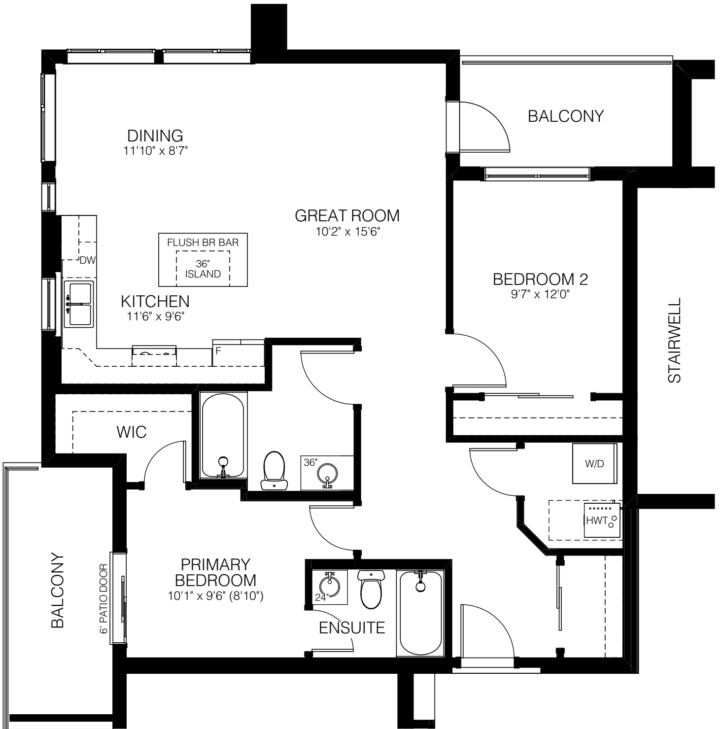
GARNET (ACCESSIBLE) UNIT TYPE 'A' BF 1043 SQFT
