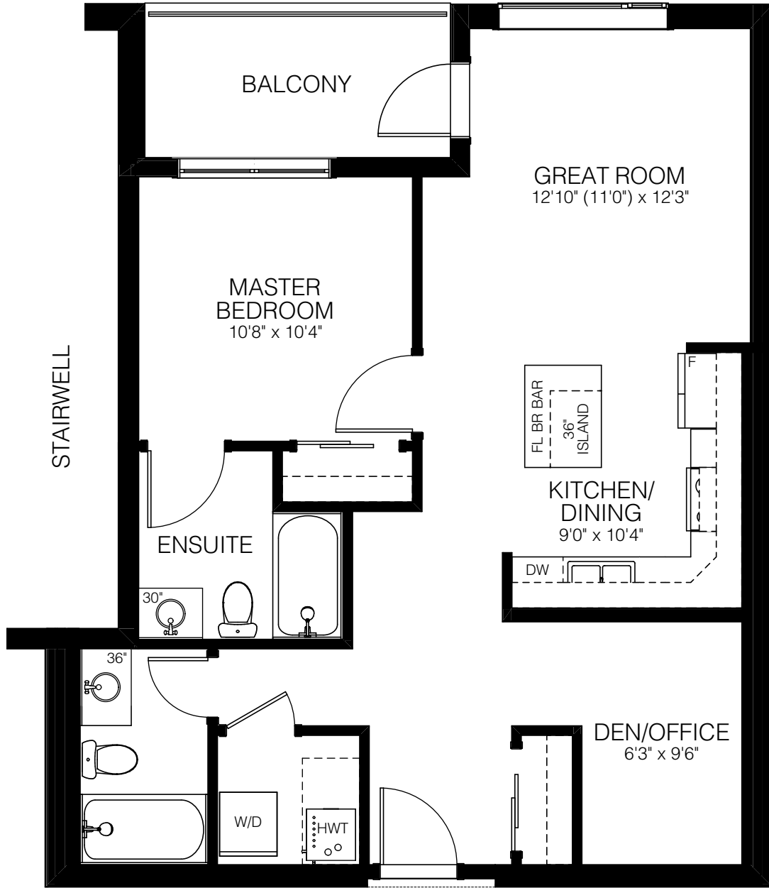
CORONATION (ACCESSIBLE) UNIT TYPE 'C' BF 796 SQFT
